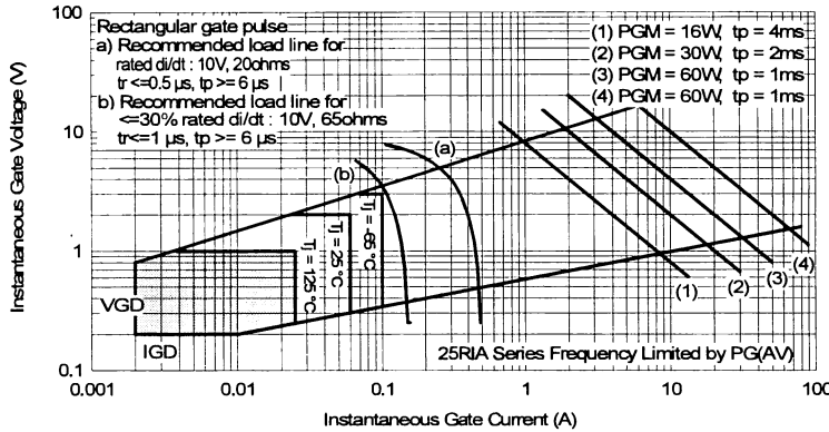
Fig. 16 - Gate Characteristics
