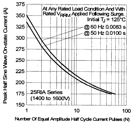
Fig. 12 - Maximum Non-Repetitive Surge Current
