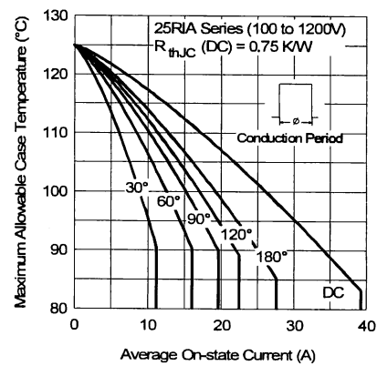
Fig. 2 - Current Ratings Characteristic
